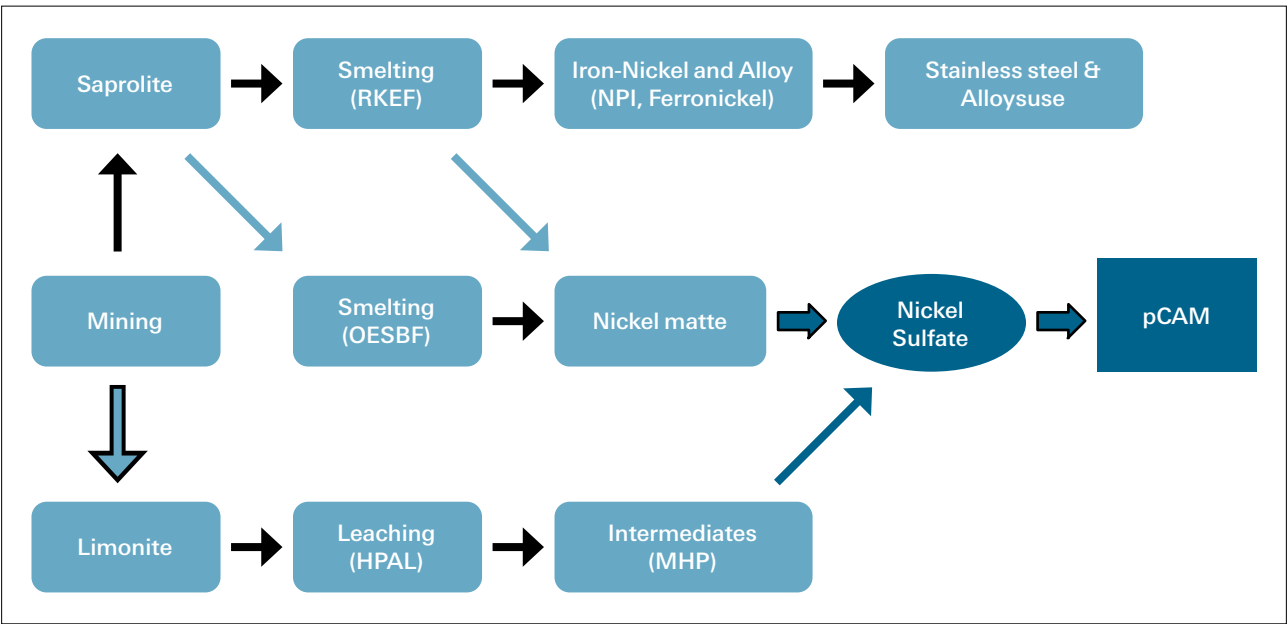
Figure 8: The value chains of nickel production and existing processing technologies in Indonesia
