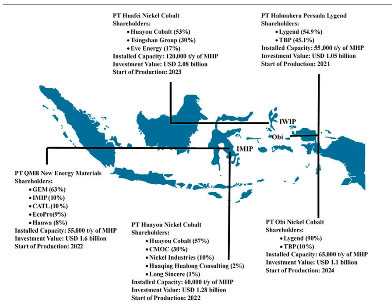
Figure 9. HPAL facilities operating in Indonesia
